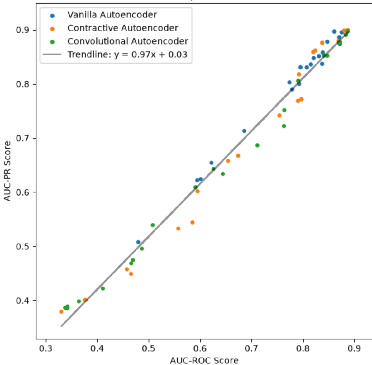
AUC Scatterplot (Model View)
